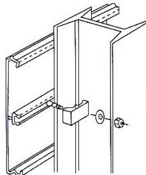
Fixing Details
