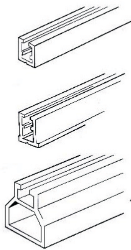
Types of Aluminum Strengthening Channels
