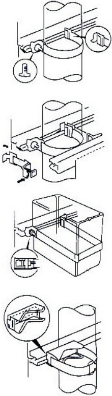
Types of steel clips
